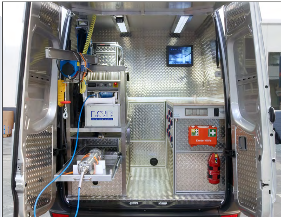
Sprinter PC 200, with manual hose reel
