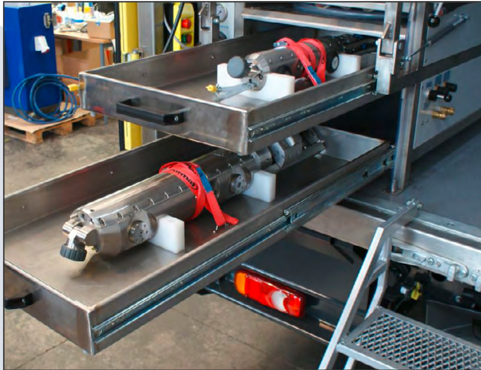
Installation – Cutting technology, universal frame drawers for robot PC150/200
